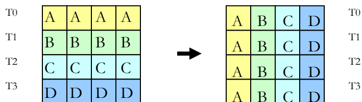
Figure 7.1-5 upc_all_exchange
